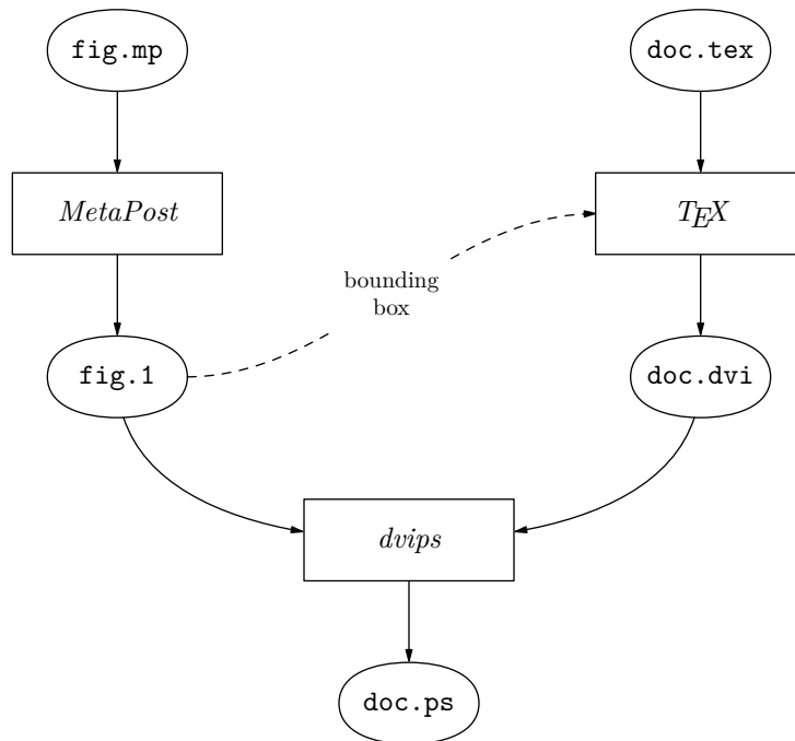
Figure 54: A diagram of the processing for a TeX document embedding MetaPost figures
