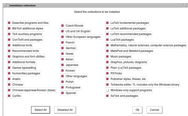
Figure 7: Collections menu
