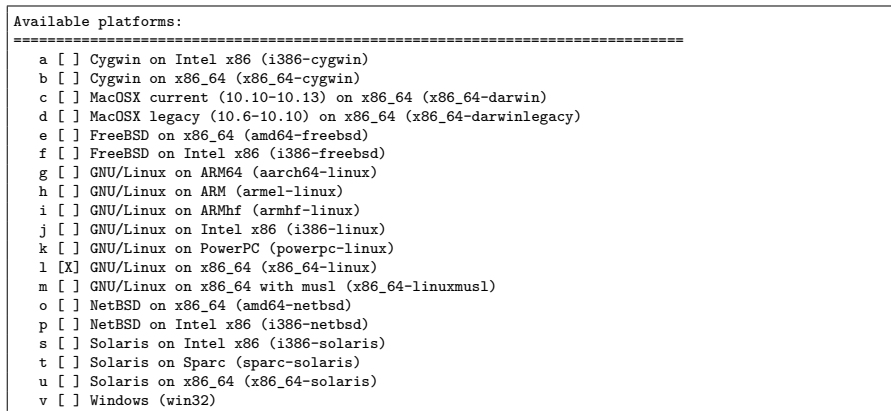
Figure 5: Binaries menu
